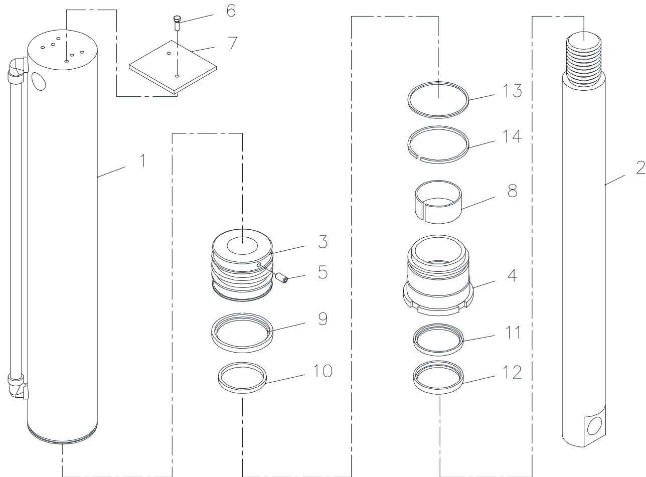
Fig. 10-2-1-1 SCS 1616 JACK CYL' ASS'Y
