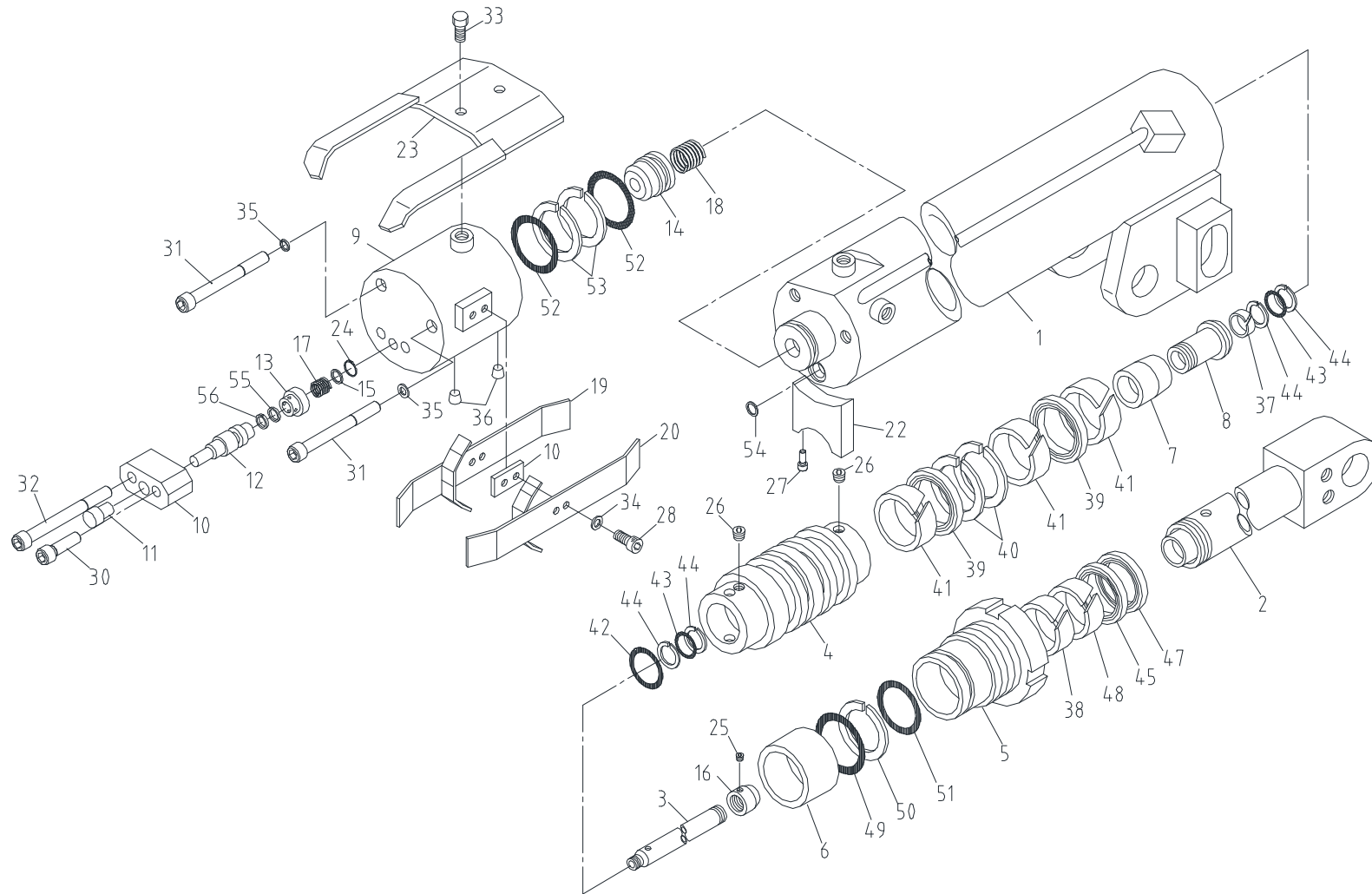
Fig. 1-1-1 SCS 1616 TELESCOPIC CYL(1st) ASS'Y
