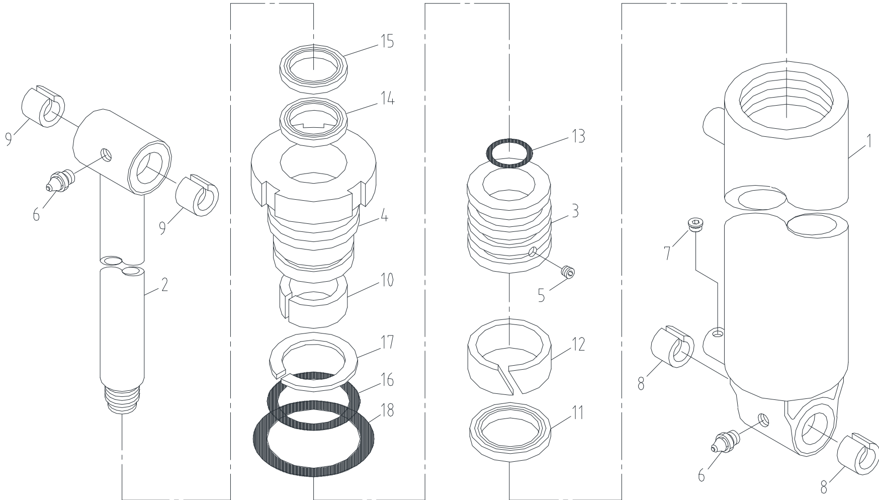
Fig. 2-1 SCS 1616 DERRICK CYL' ASS'Y
