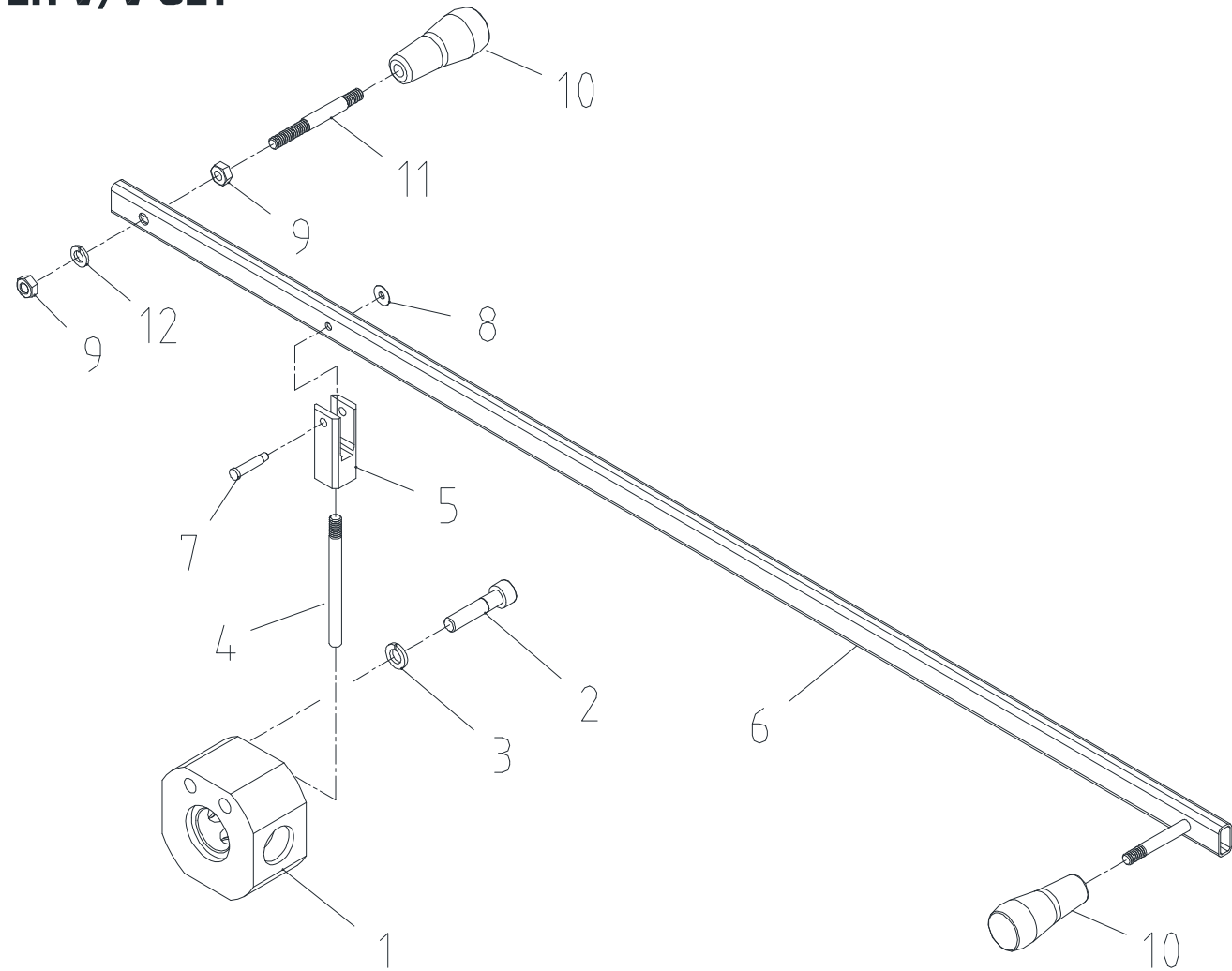
Fig. 3-1 SCS 1616 DIVERter V/V SET
