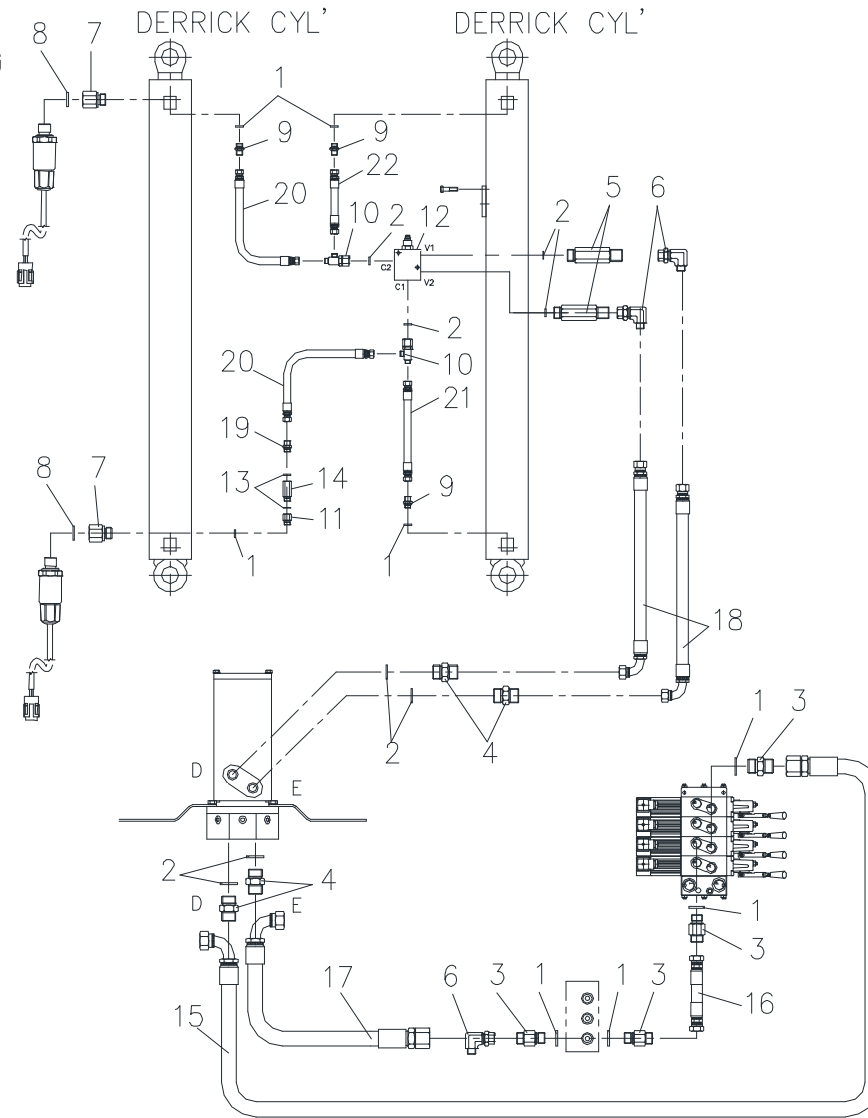
Fig. 5-3 SCS 1616 DERRICK PIPING
