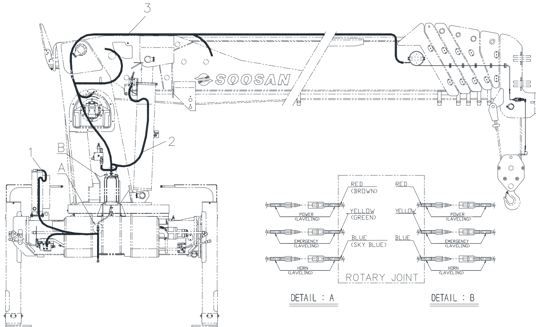
Fig. 8 SCS 1616 WIRING ASS'Y
