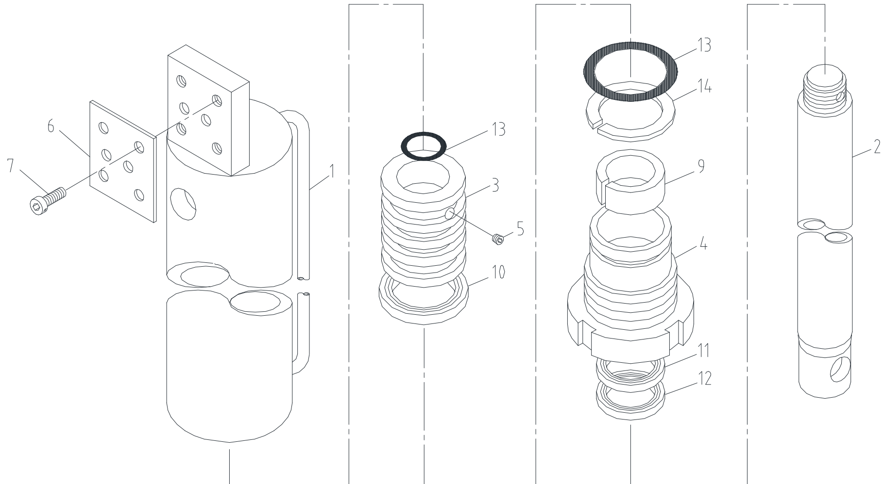
Fig. 4-2 SCS 1616 JACK CYL' ASS'Y
