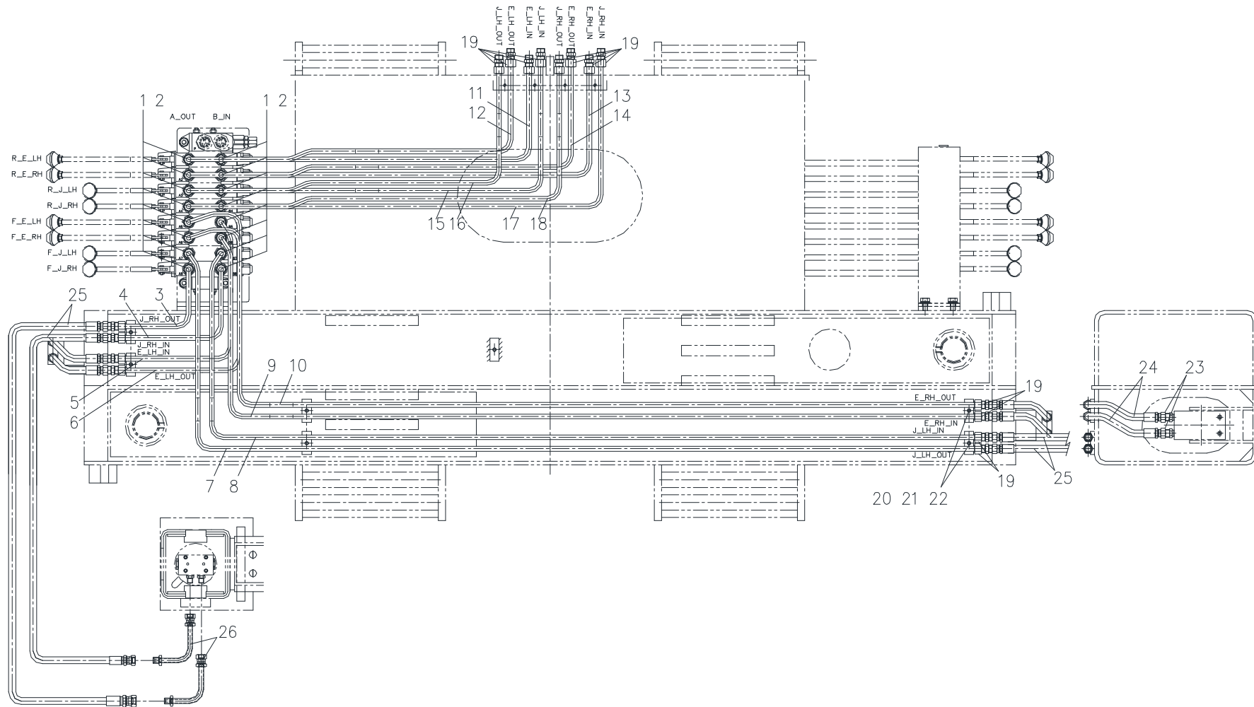
Fig. 5-6 SCS 1616 OUTRIGGER PIPING
