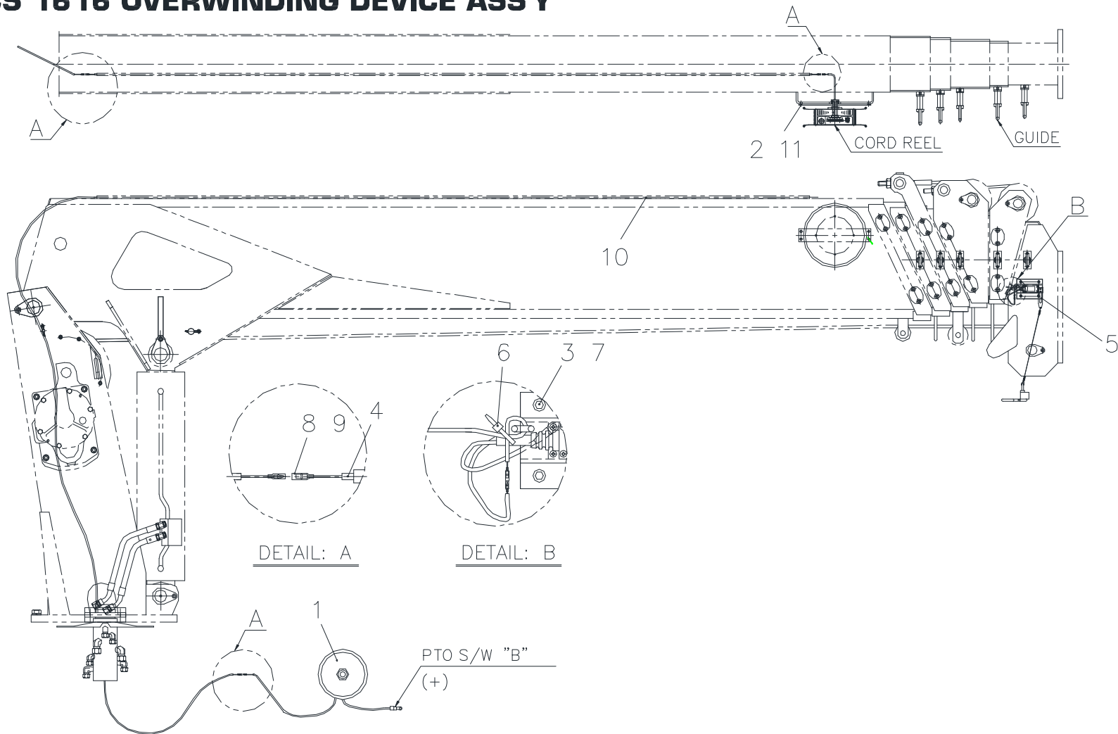
Fig. 13 SCS 1616 OVERWINDING DEVICE ASS'Y
