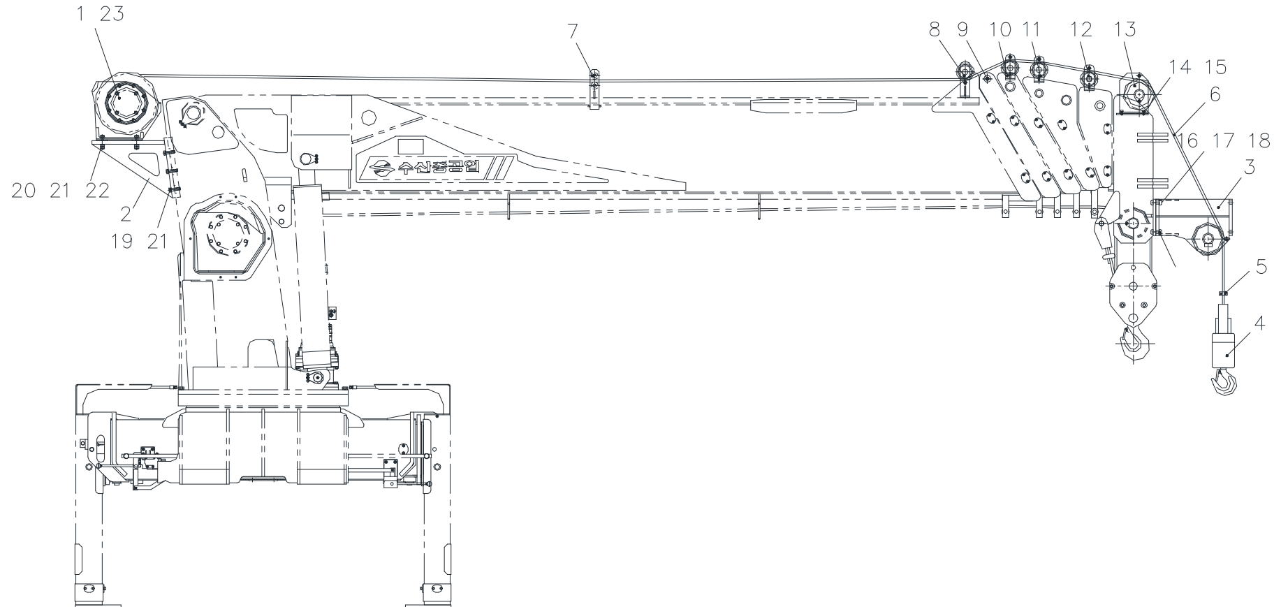
Fig. 11 SCS 1616 SUB WINCH ASS'Y
