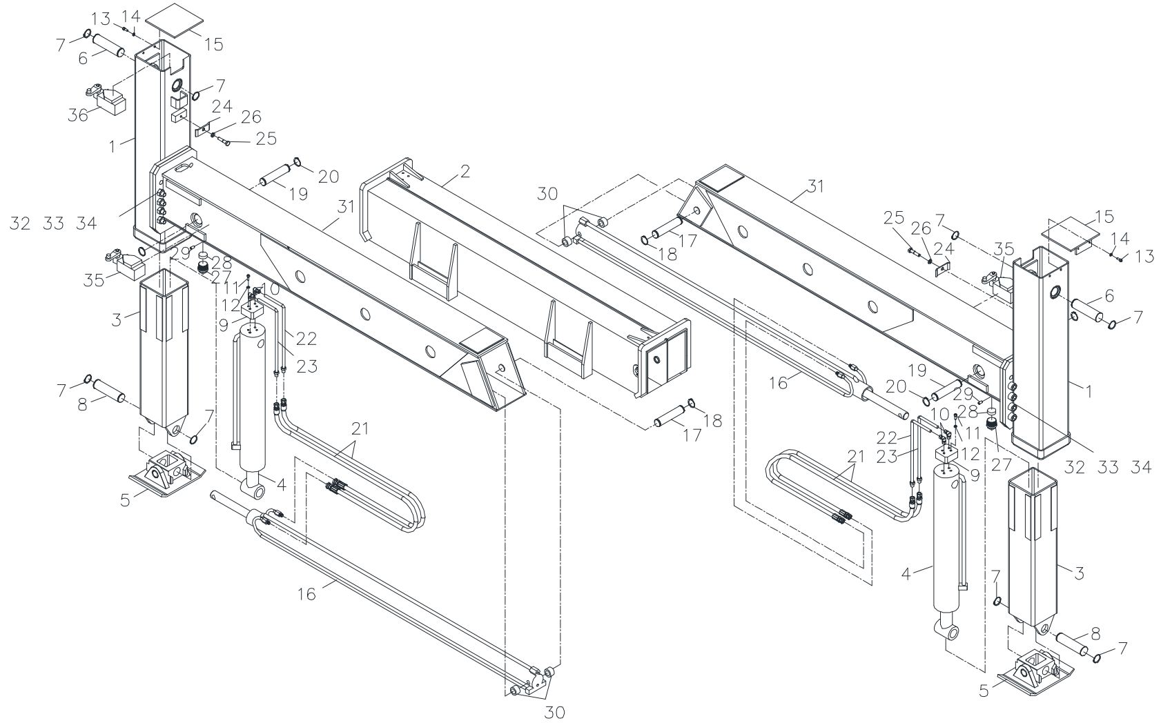
Fig. 10-2-1 SCS 1616 REAR OUTRIGGER ASS'Y
