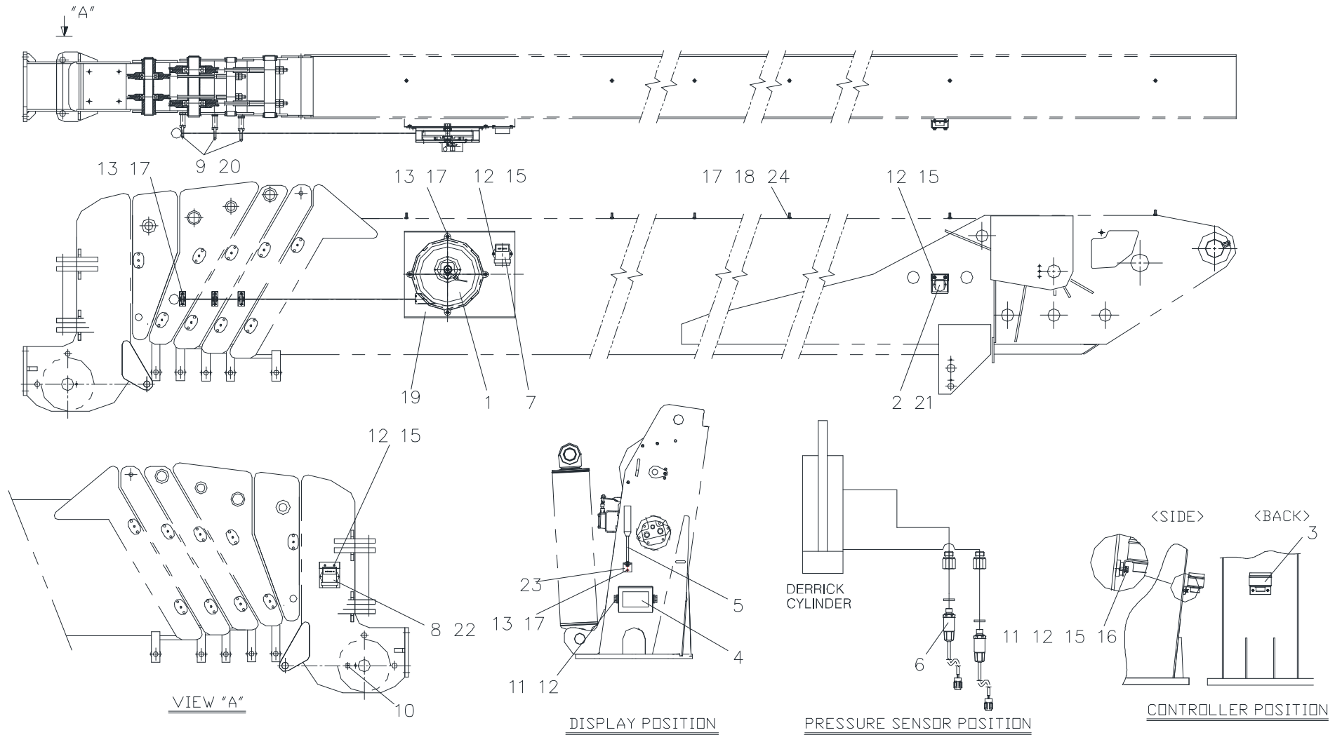
Fig. 9 SCS 1616 AML OVERWINDING SETTING DRAWING
